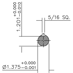
SECTION THROUGH 'X'
