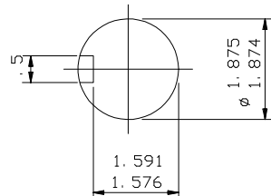
ENLARGED VIEW OF SHAFT EXTENSION (SCALE 1:2)
