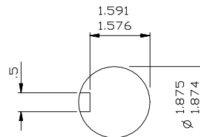
SECTION THROUGH SHAFT EXTENSION. (SCALE 1:2).
