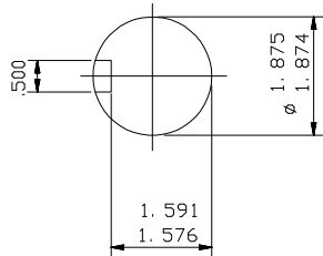
ENLARGED VIEW OF SHAFT EXTENSION
