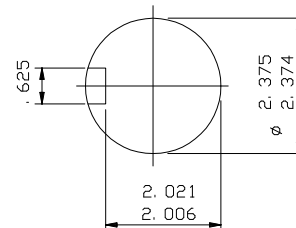
ENLARGED VIEW OF SHAFT EXTENSION (SCALE 1: 2)
