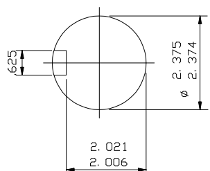
ENLARGED VIEW OF SHAFT EXTENSION (SCALE 1:20)
