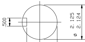
ENLARGED VIEW OF SHAFT EXTENSION (SCALE 1:2)
