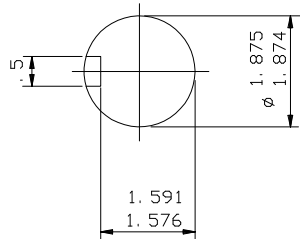
ENLARGED VIEW OF SHAFT EXTENSION (SCALE 1: 2)
