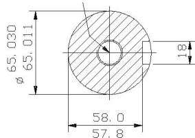
SECTION THROUGH SHAFT EXTENSION (SCALE 1: 2.5)
