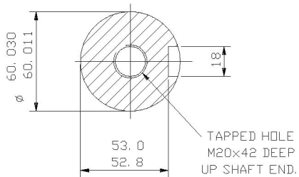
SECTION THROUGH SHAFT EXTENSION
