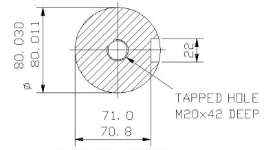
SECTION THROUGH SHAFT EXTENSION (SCALE 1: 2)
