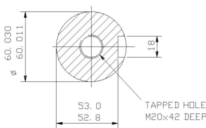
SECTION THROUGH SHAFT EXTENSION (SCALE 1: 2)
