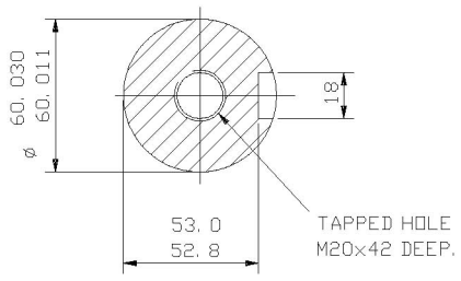
SECTION THROUGH SHAFT EXTENSION (SCALE 1:2)
